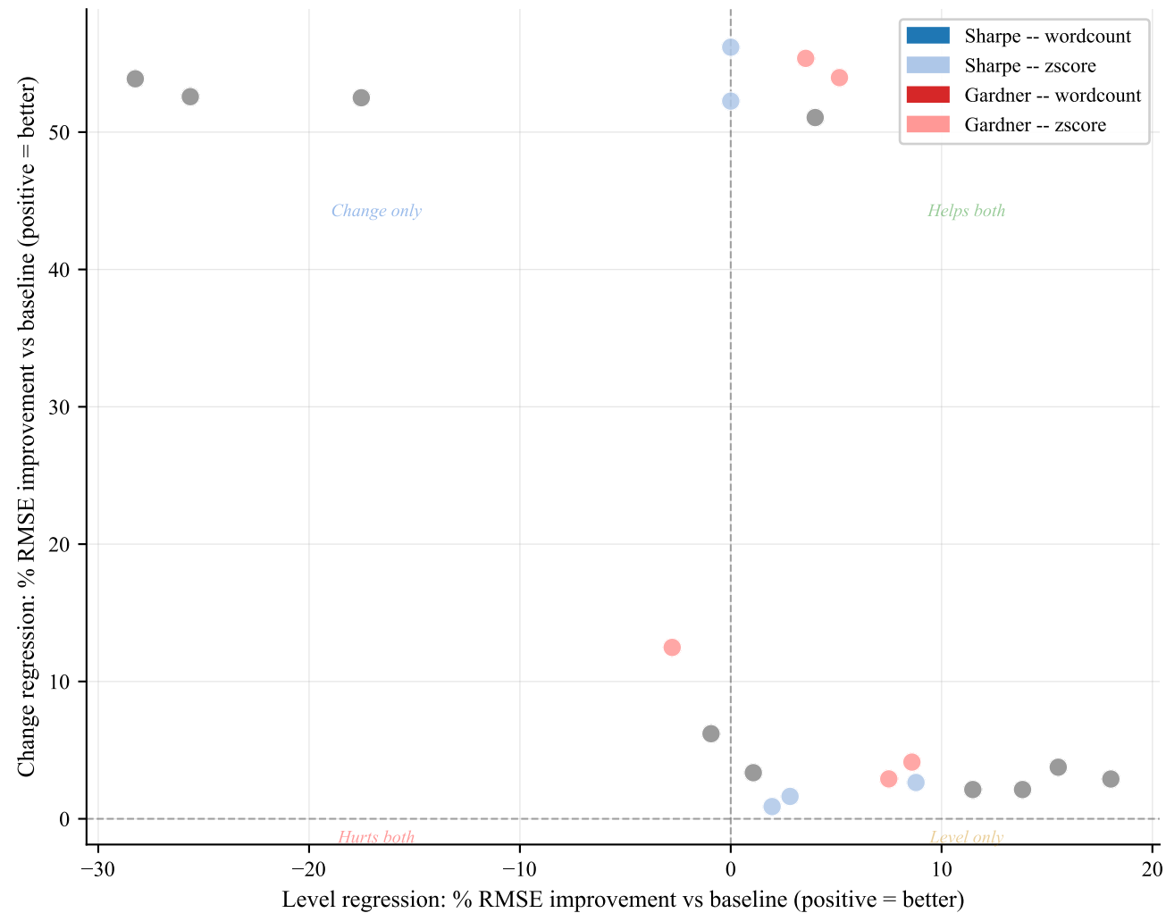
Level vs Change OOS Improvement (80% init) Each point = one dictionary x doc-type x norm combo
